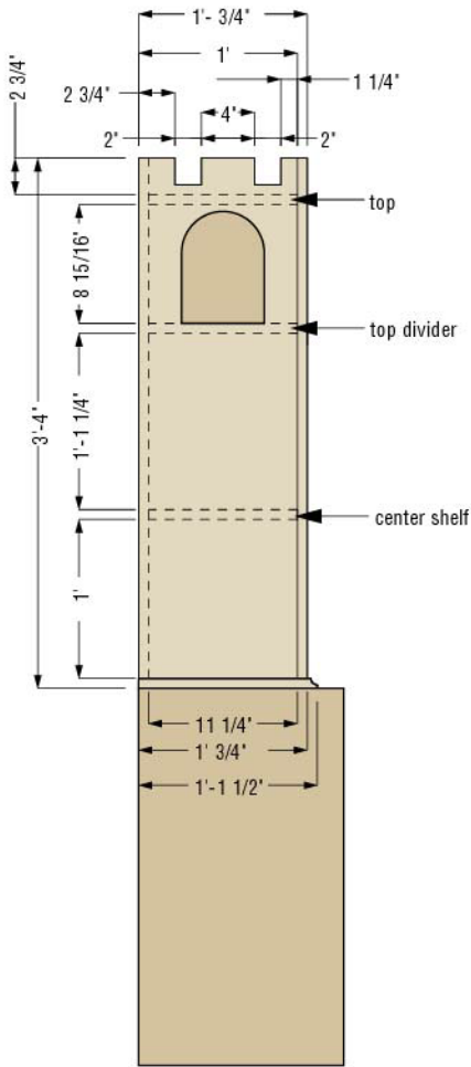
Side View
