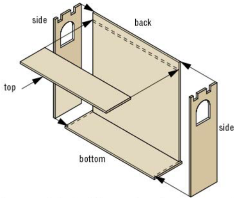
1. Assemble bottom, back, top, and sides.
