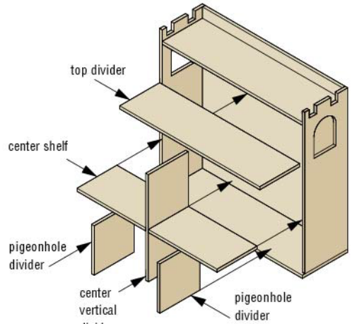
2. Assemble shelving.
